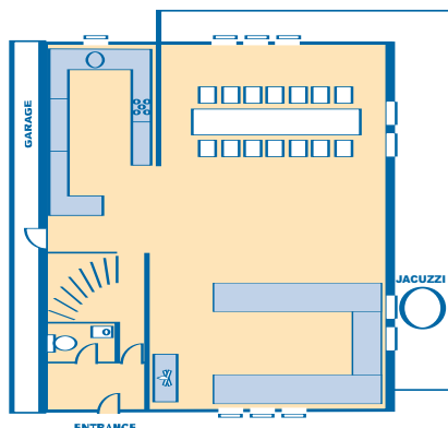
CHALET FOEHN MIDDLE FLOOR
